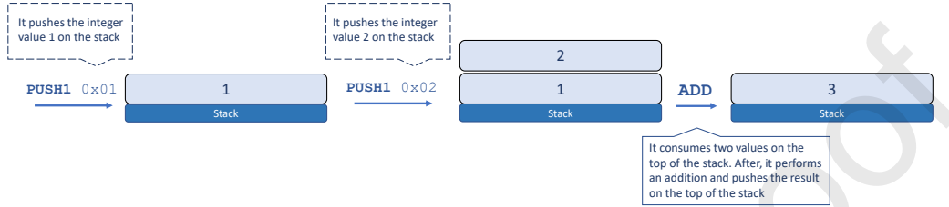
Figure 1: Execution of a EVM bytecode that computes the addition of two integers.
